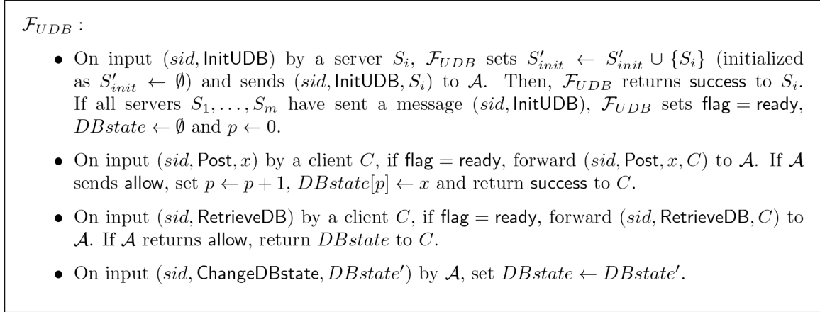
Figure 6: The functionality \mathcal{F}_{UDB} models an unreliable database and interacts with a set of n clients, a set of m servers and the adversary \mathcal{A} .
