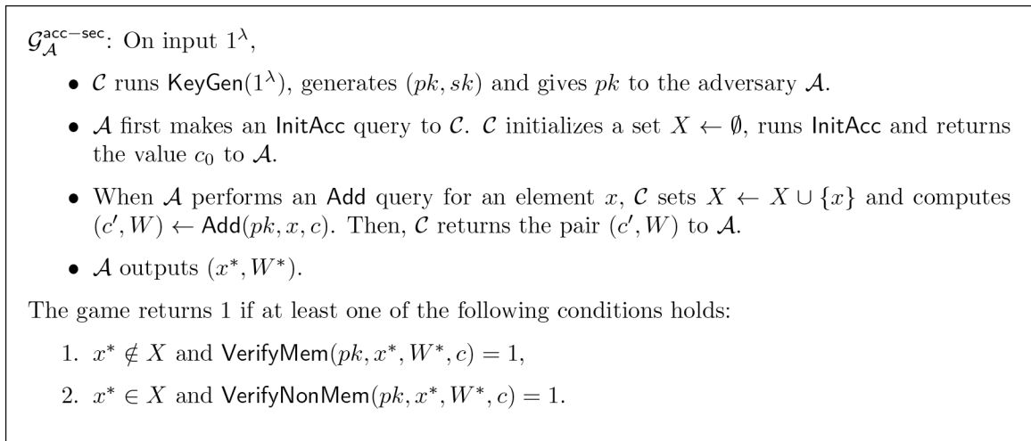
Figure 1: The security game between the adversary \mathcal{A} and a challenger \mathcal{C} , where \mathcal{C} plays the roles of both T and T_{acc} .
