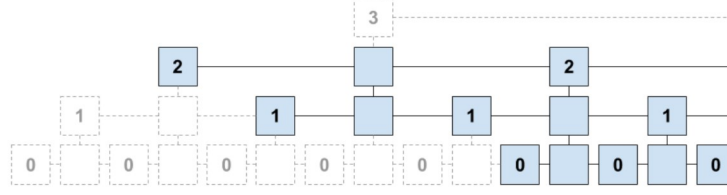
Fig. 3. NIPoPoW prefix \pi for m = 3 .
