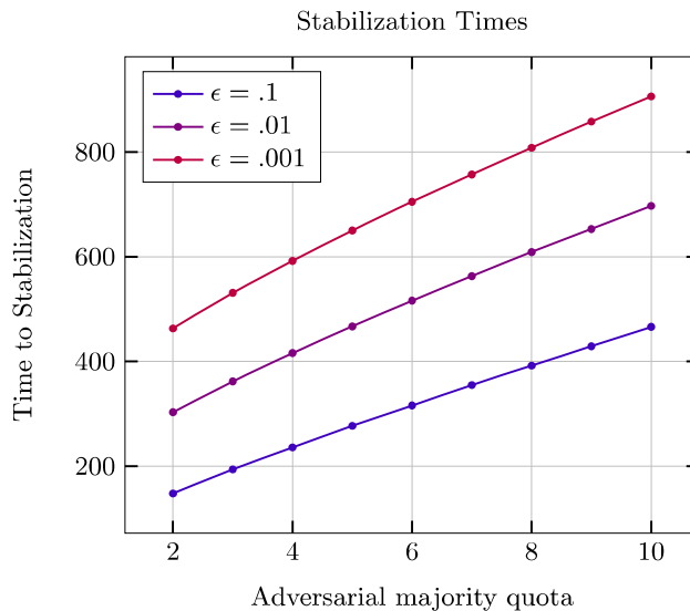
Fig. 3. Graphs of the time necessary for a PoW blockchain to stabilize (with prescribed error) with various spike quotas. These plots correspond to a 10% adversary, \Delta = 3 , and a success probability p chosen so that the expected number of honest successes over 7 = 2\Delta + 1 rounds is 1. The three graphs show target errors of 1/10, 1/100, and 1/1000 over a range of adversarial spike quotas.
