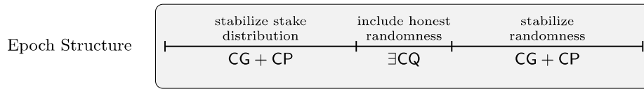
Fig. 8. Illustration of the three different intervals of an epoch for the inductive argument underlying Genesis.
