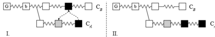
Fig. 8. Adversarial fork chain C_A and chain C_B of an honest party. Thorny blocks are colored black. Dashed arrows represent interlink pointers. After the protocol update when an adversarially generated block is sewed from C_B into the adversary's suffix proof the verifier perceives C_A as longer and C_B as shorter. I: The real picture of the chains. II: Equivalent picture from the verifier's perspective considering the suffix proof for each chain.
