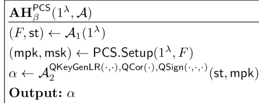
Fig. 2: The Strong Attribute Hiding Game for PCS.
